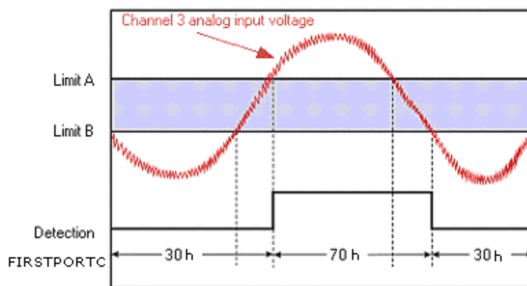
Figure 26. Channel 3 in hysteresis mode
