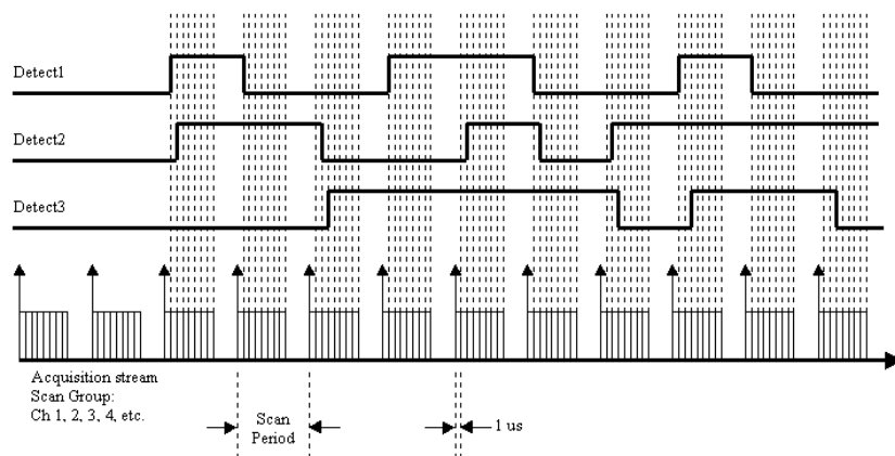
Figure 23. Example diagram of detection signals for channels 1, 2, and 3
