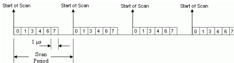
Figure 7. Analog channel scan of voltage inputs example
