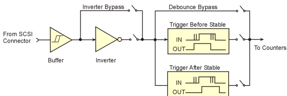
Figure 12. Debounce model block diagram
